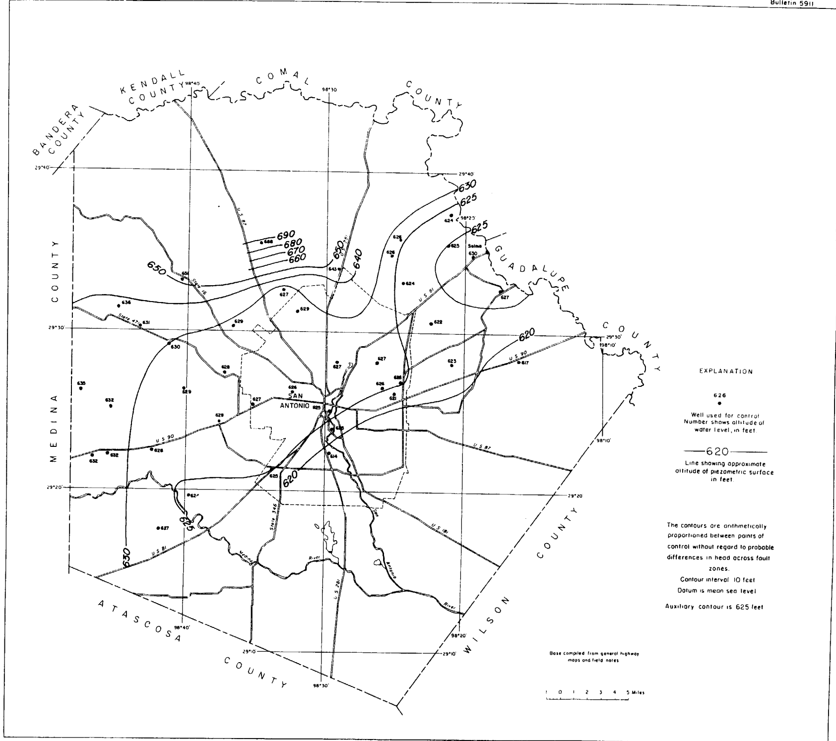
FIGURE 8 - Contour map of the piezometric surface of the Edwards and associated limestones, Bexar County, Texas, January 1957
