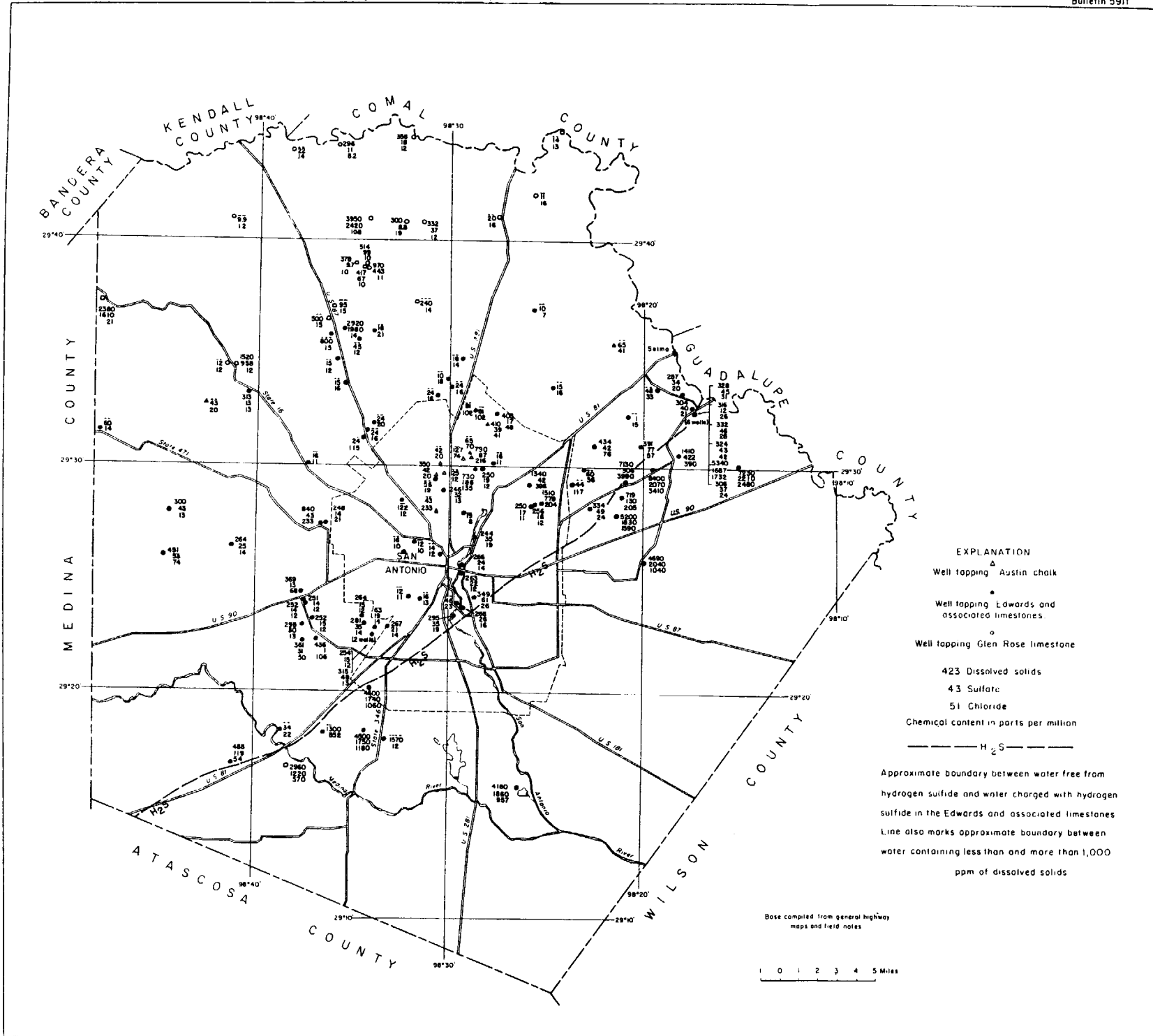
FIGURE 10 - Map showing dissolved solids, sulfate, and chloride in the ground water in Bexar County, Texas.
