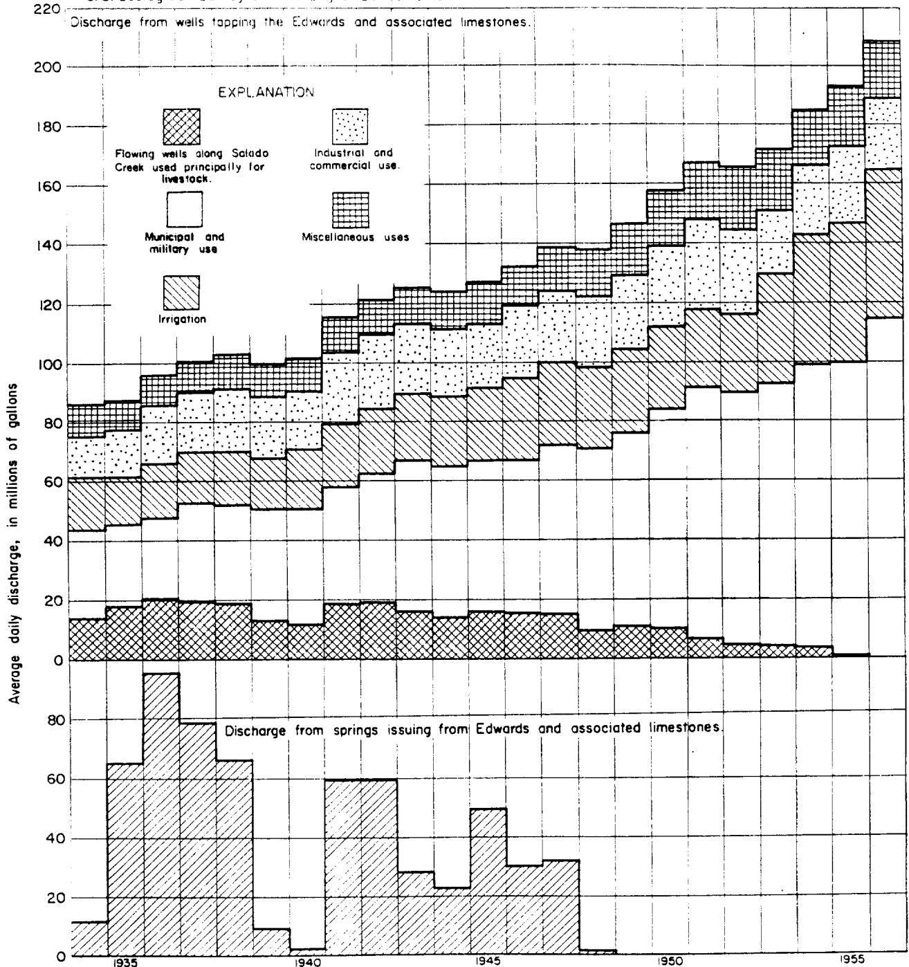
FIGURE 3. Graph showing daily discharge from wells and springs in the Edwards and associated limestones, by type of use, 1934-56.
