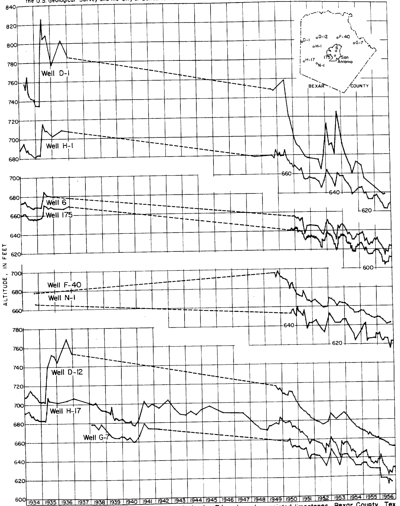
FIGURE 2.- Hydrographs of representative wells in the Edwards and associated limestones, Bexar County, Tex.
