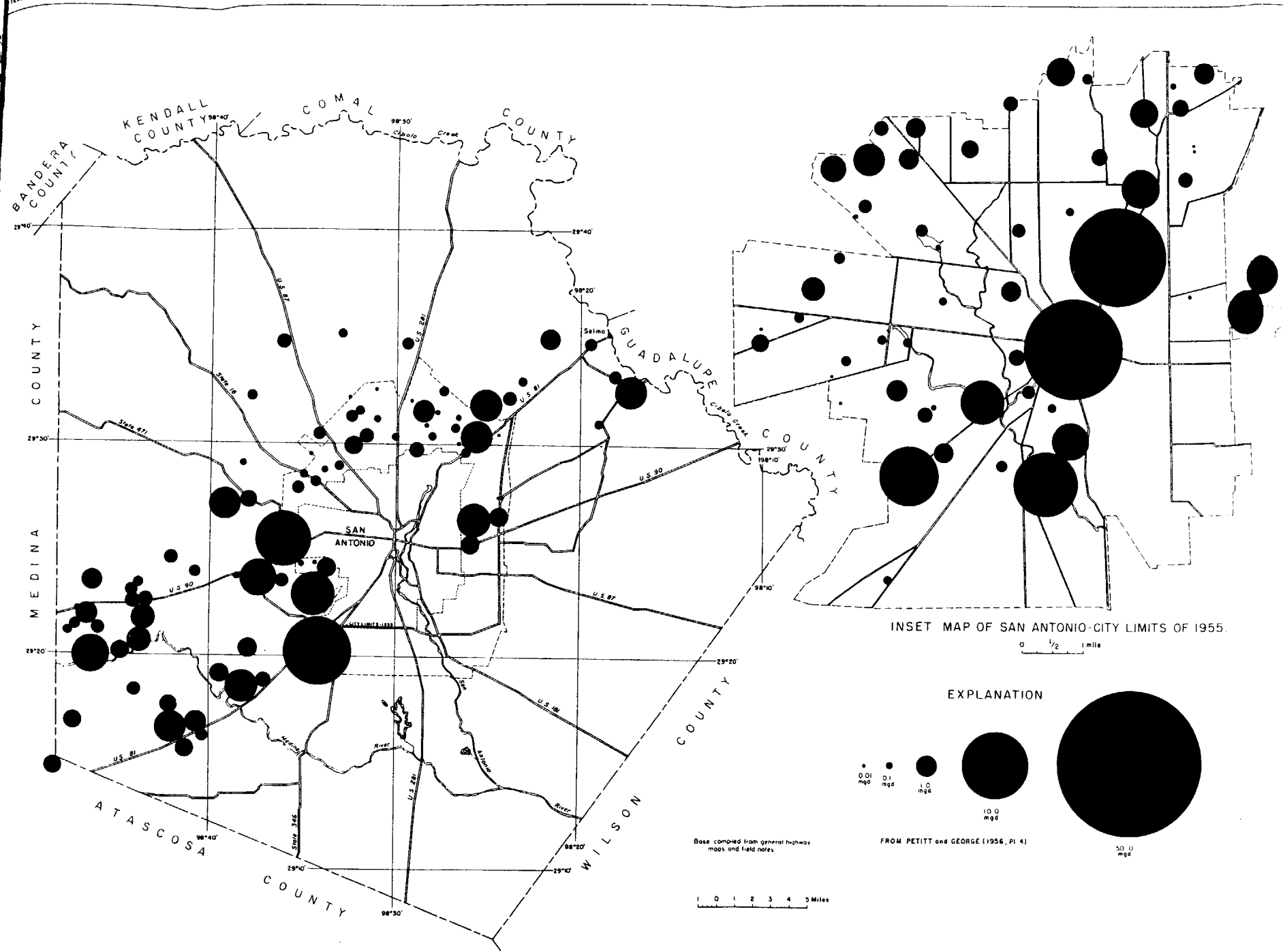
FIGURE 4 - Map showing distribution of discharge from wells and springs in the Edwards and associated limestones, Bexar County, Texas, 1954
