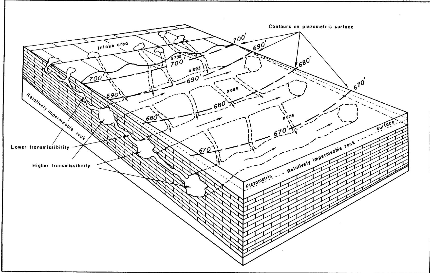
FIGURE 9 - Hypothetical diagram showing how water in the cavernous Edwards and associated limestones may flow approximately parallel to the trend of the regional contours on the piezometric surface.
