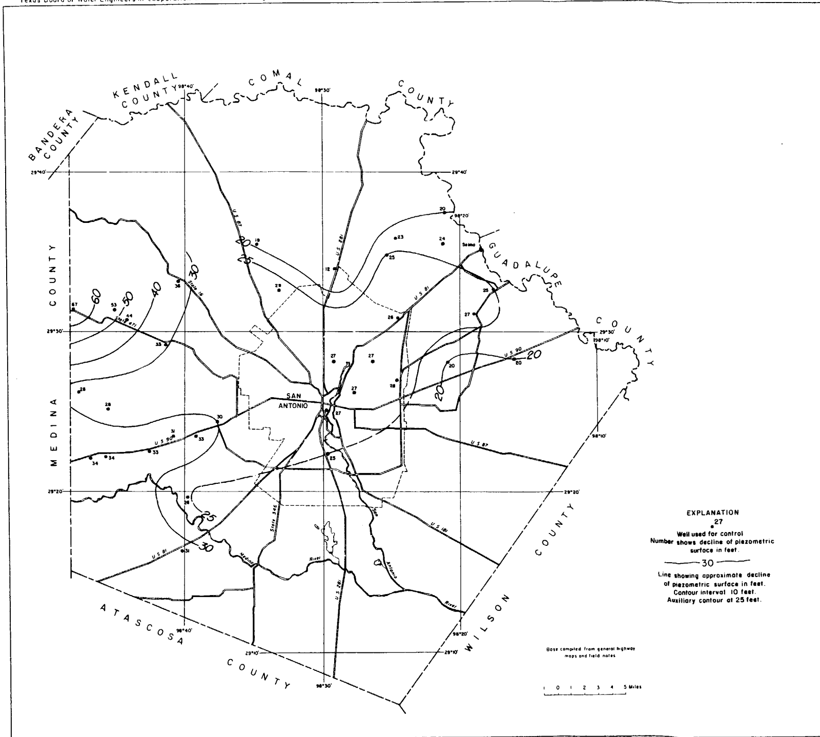
FIGURE 12 Contour map showing decline of the piezometric surface of the Edwards and associated limestones, Bexar County, Texas, 1933-1954 Contours are based on measurements made from August 1933 to January 1954.
