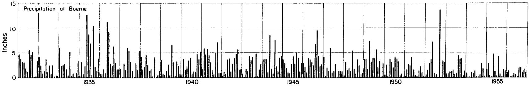
FIGURE 11. Hydrograph of well 26 and monthly precipitation at San Antonio and at Boerne, Kendall County. (Precipitation data from U.S. Weather Bureau.)
