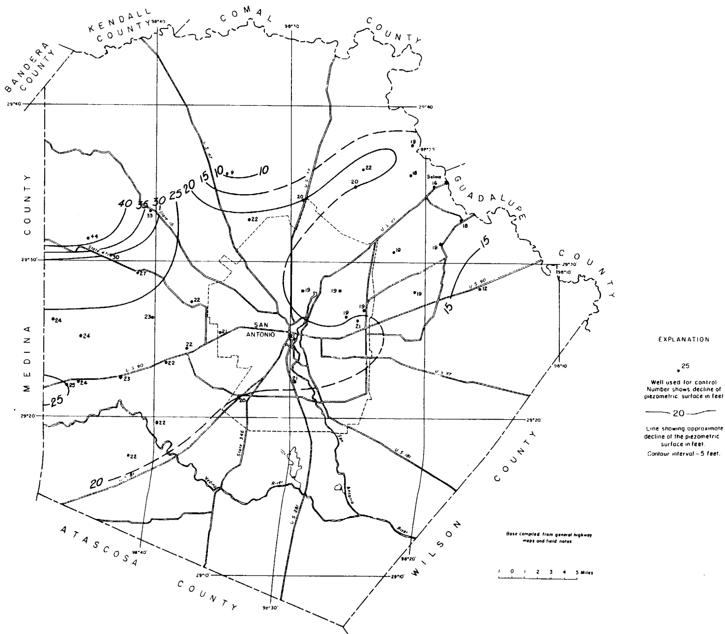
FIGURE 13 - Contour map showing decline of the piezometric surface of the Edwards and associated limestones, Bexar County, Texas - January 1954, January, 1957
