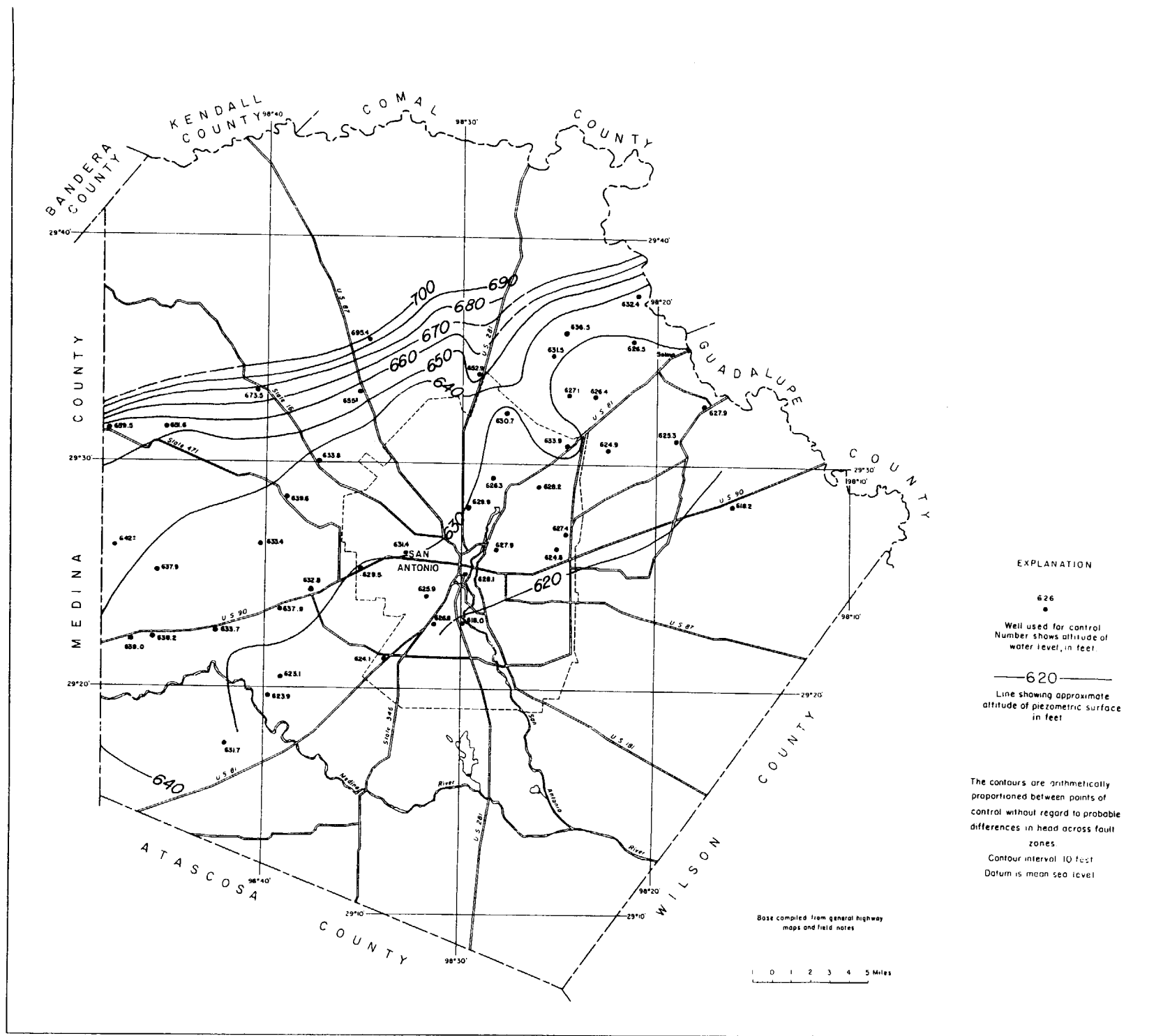
FIGURE 7 - Contour map of the piezometric surface of the Edwards and associated limestones, Bexar County, Texas, August 1954
