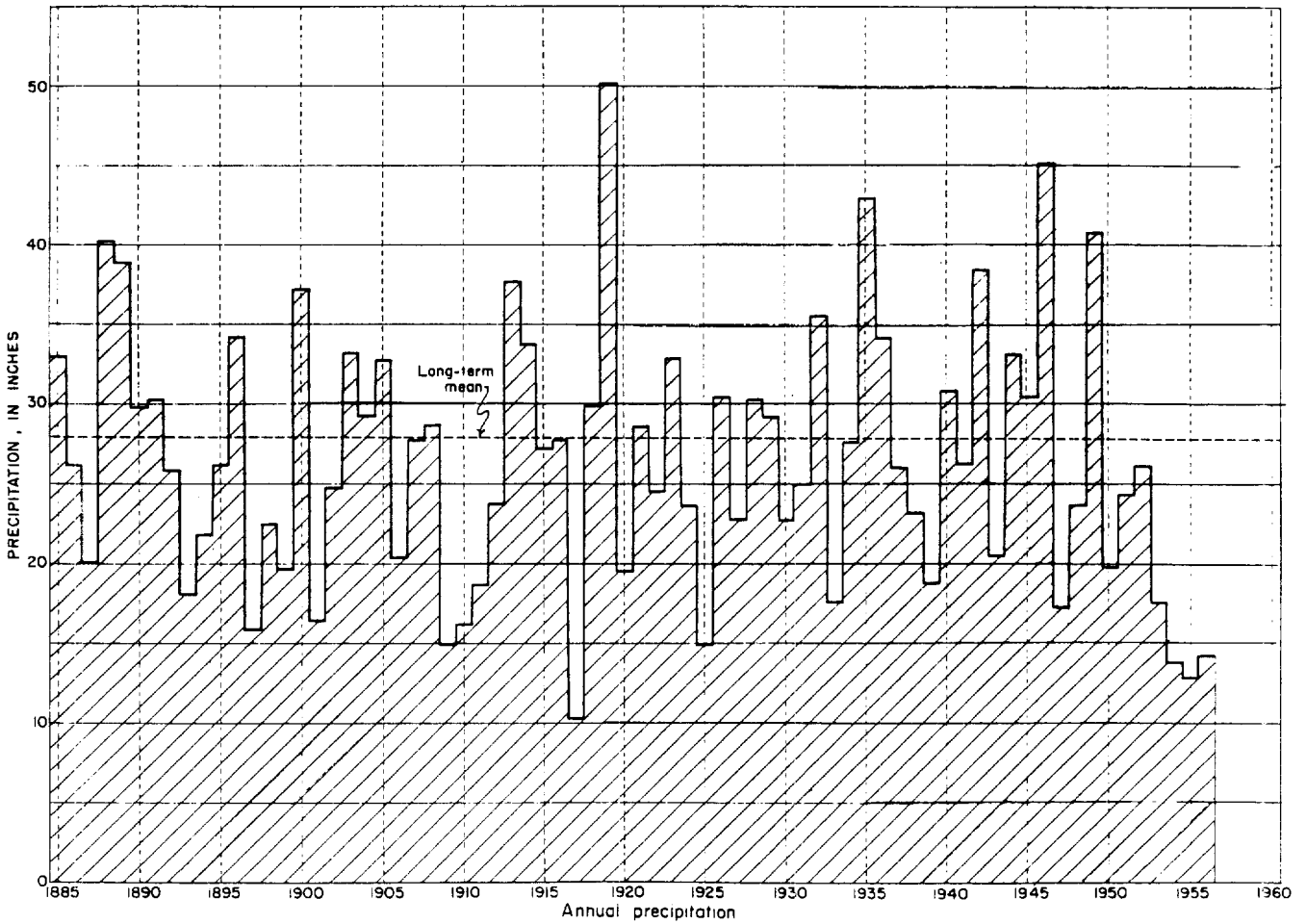
FIGURE 1a.—Mean monthly temperature and precipitation and annual precipitation at San Antonio Airport, Bexar County, Tex.
