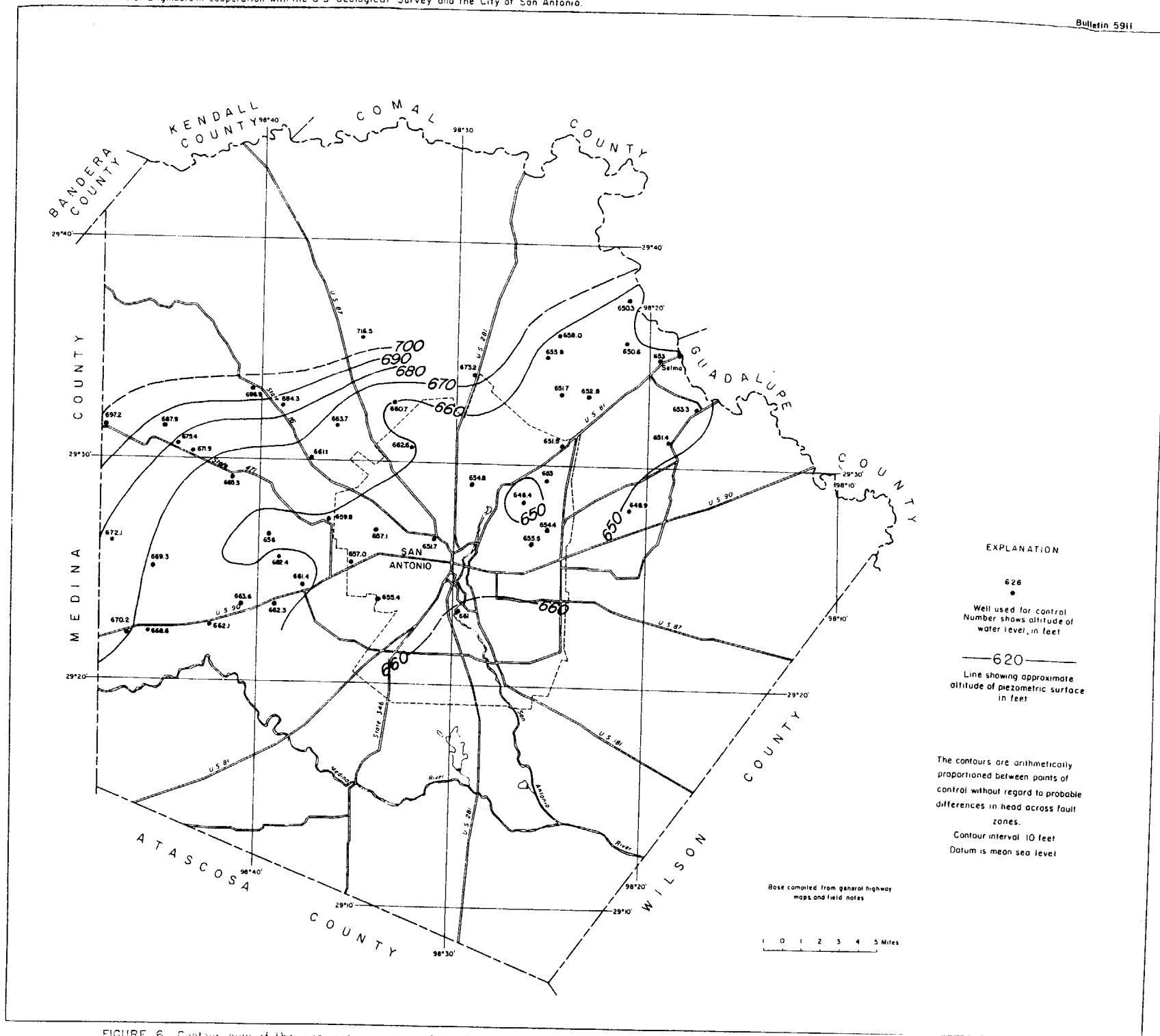
FIGURE 6 Contour map of the piezometric surface of the Edwards and associated limestones, Bexar County, Texas, January 1952.
