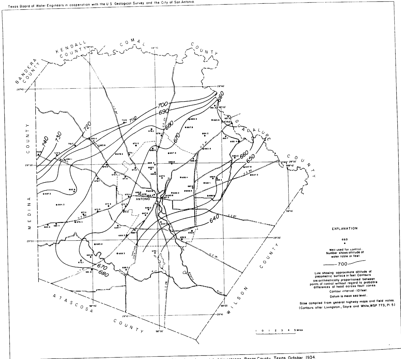
FIGURE 5 - Contour map of the piezometric surface of the Edwards and associated limestones, Bexar County, Texas, October 1934.
