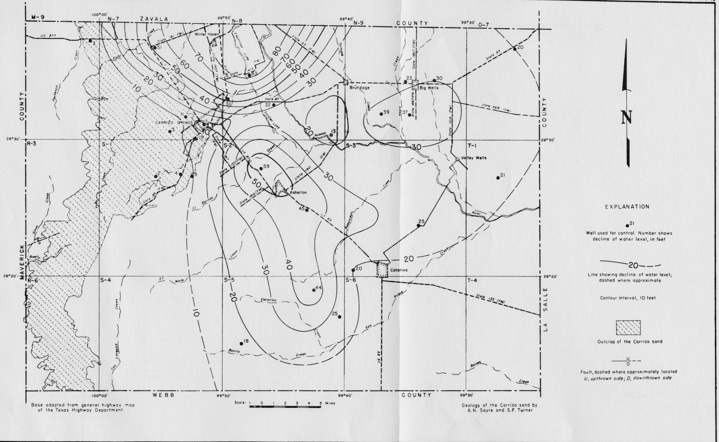
DECLINE OF WATER LEVELS IN WELLS IN THE CARRIZO SAND, DIMMIT COUNTY, TEXAS, 1938 - 48.
