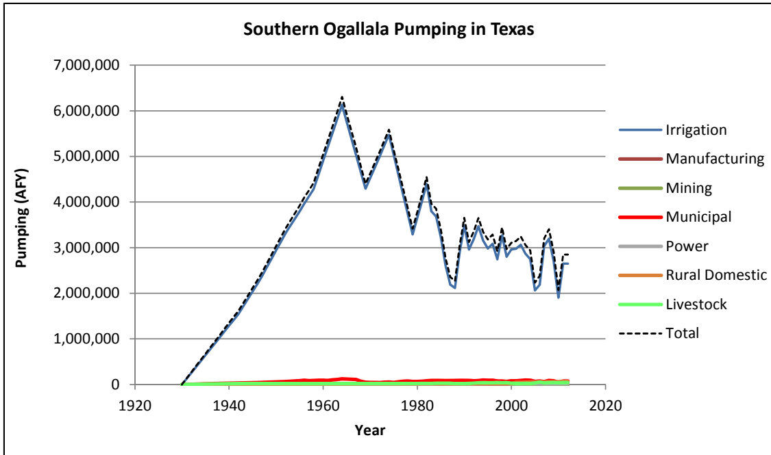
Figure 4.7.19 Estimated pumping in acre-feet per year in the Texas portion of the Southern Ogallala Aquifer.
