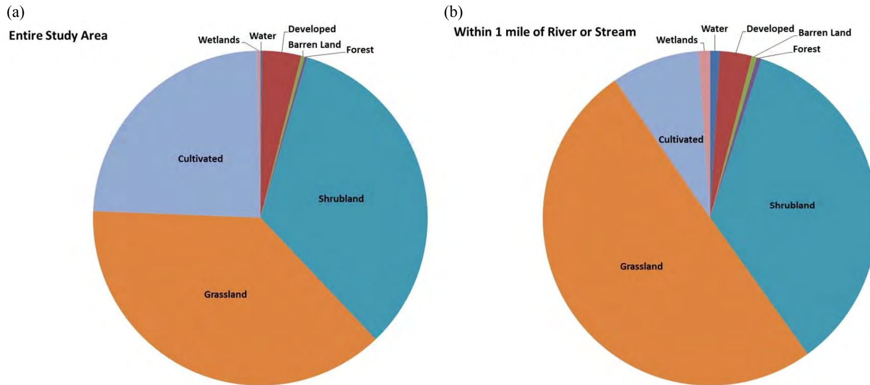
Figure 4.7.3 Land use distribution in the (a) entire study area and (b) within 1 mile of a river or stream.
