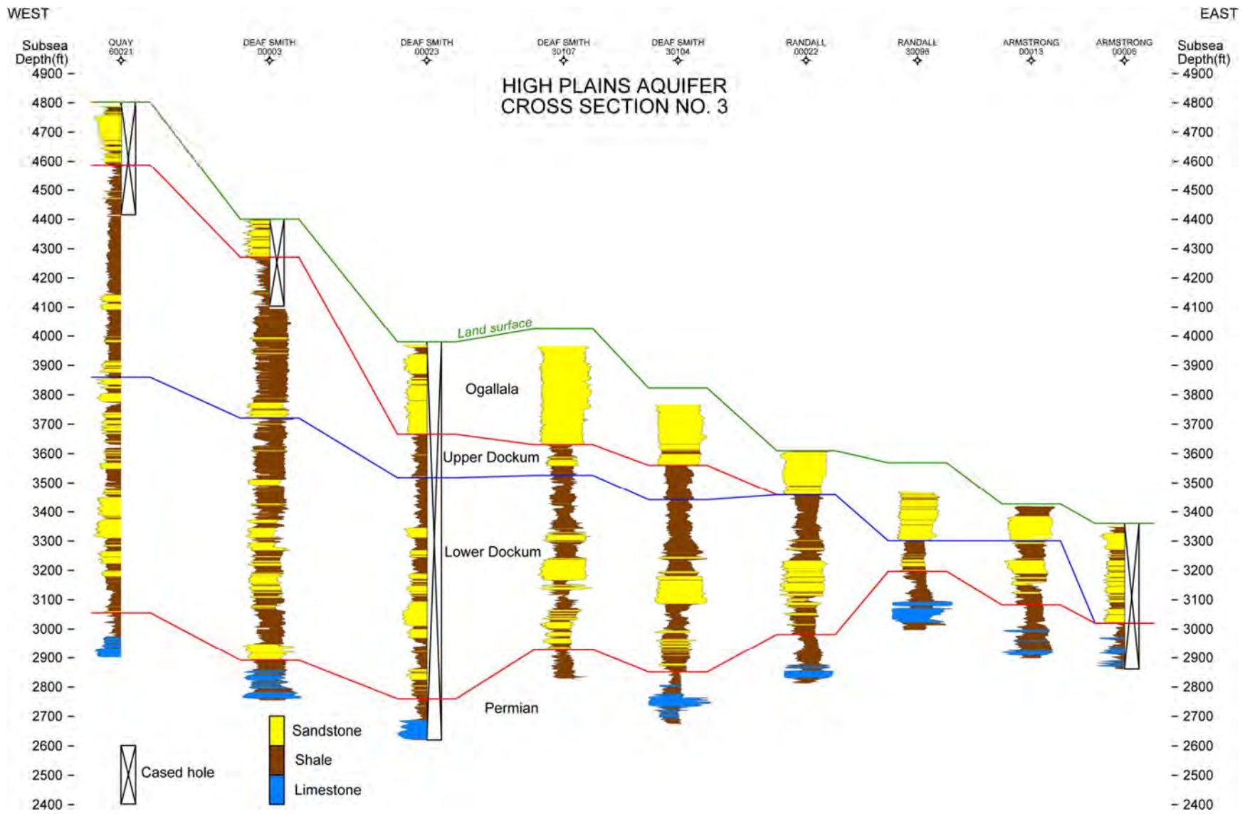
Figure 4.2.5 Cross-section #3.
