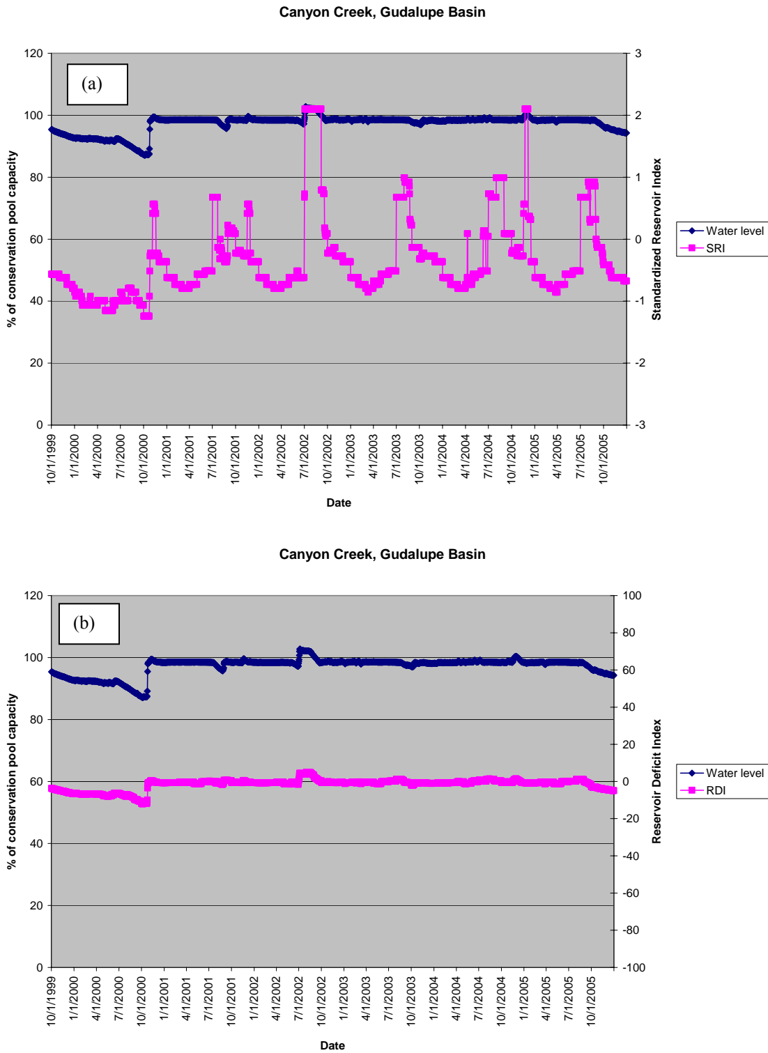
Figure 37 a) Standardized Reservoir Index (SRI) b) Reservoir Deficit Index (RDI) for Canyon Lake Reservoir, Guadalupe basin (2000–2005)
