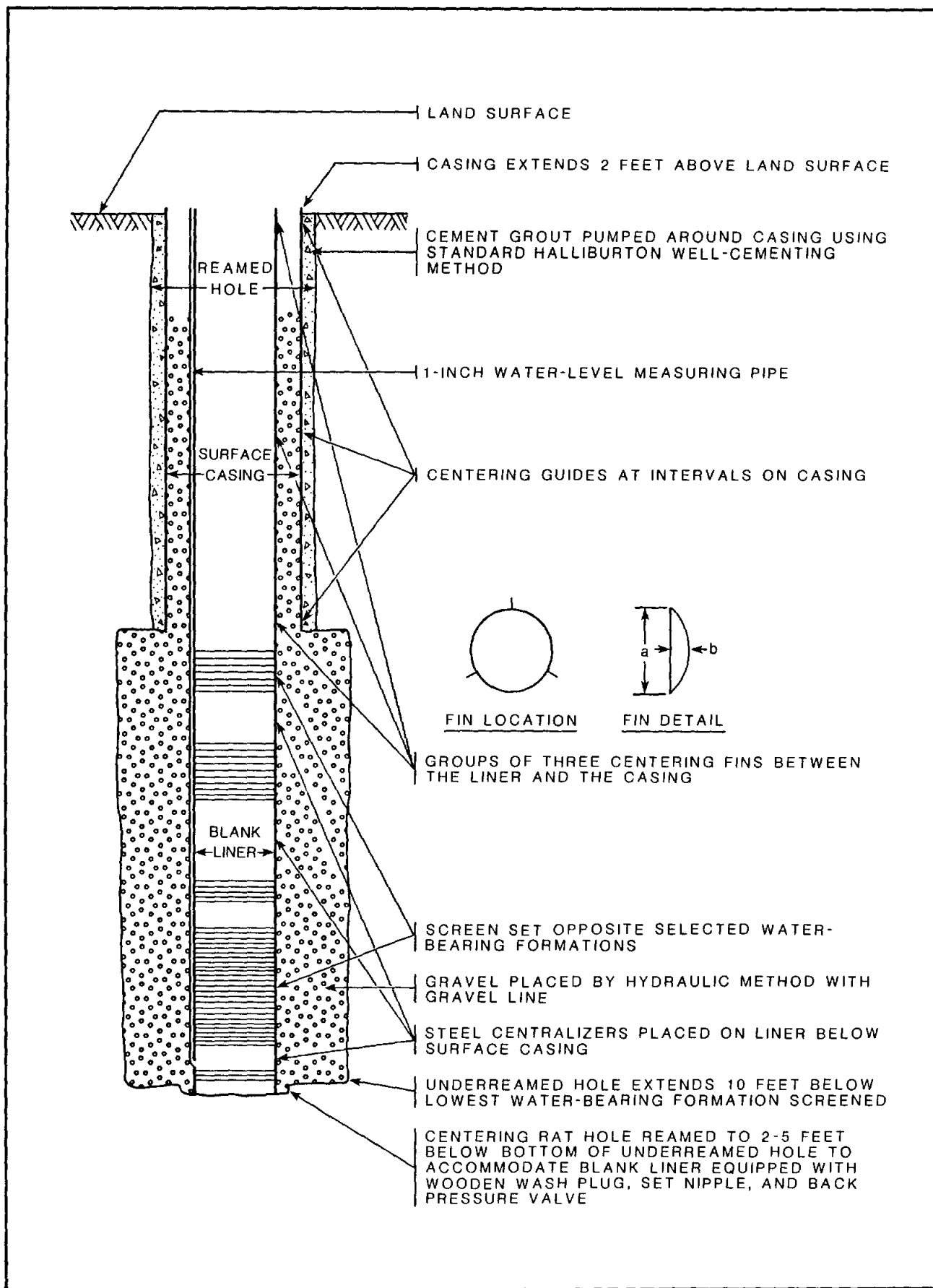
TYPICAL GRAVEL WALL WELL
