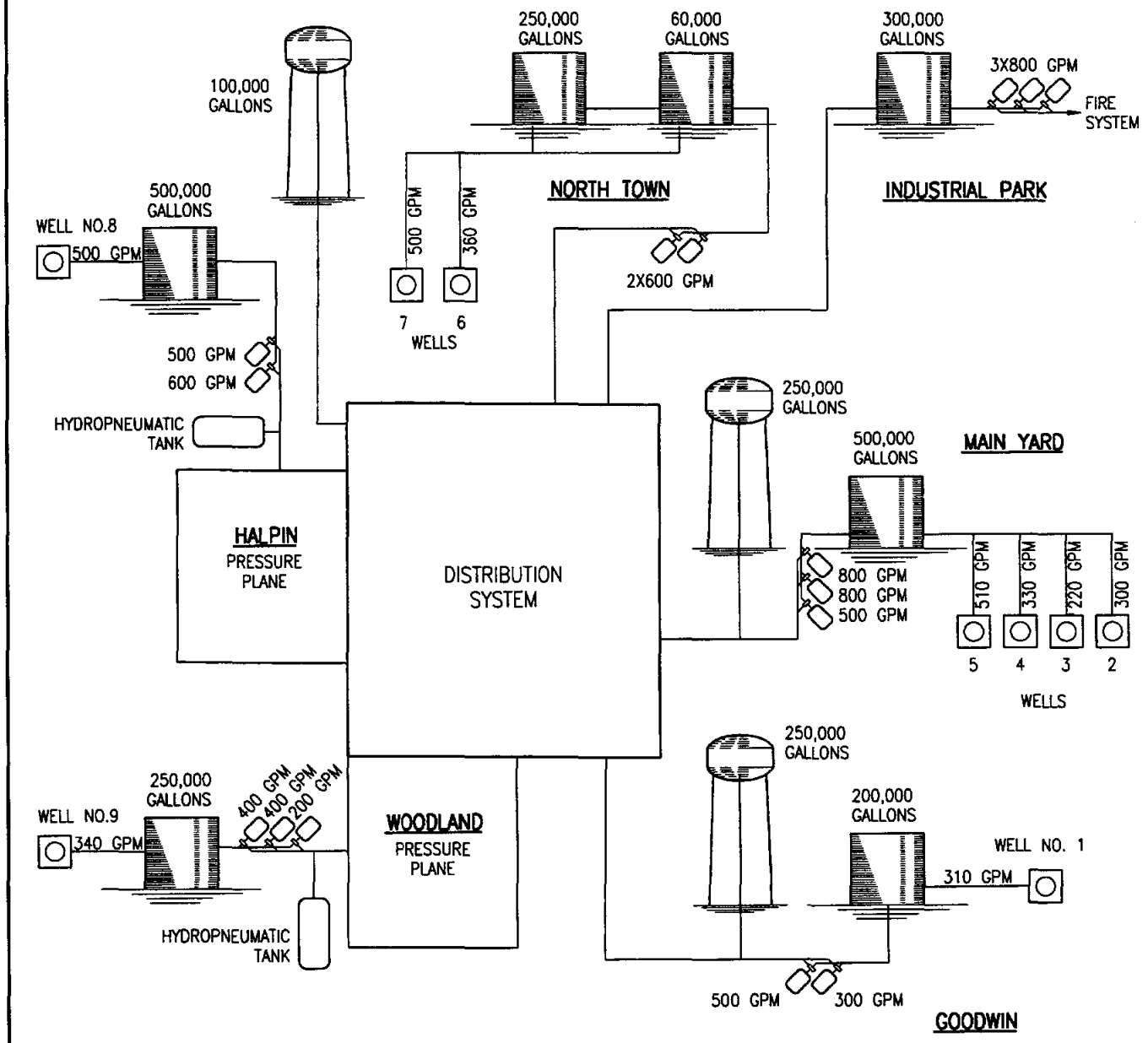
FIGURE 4.7-1 CITY OF PLEASANTON WATER SYSTEM SCHEMATIC
