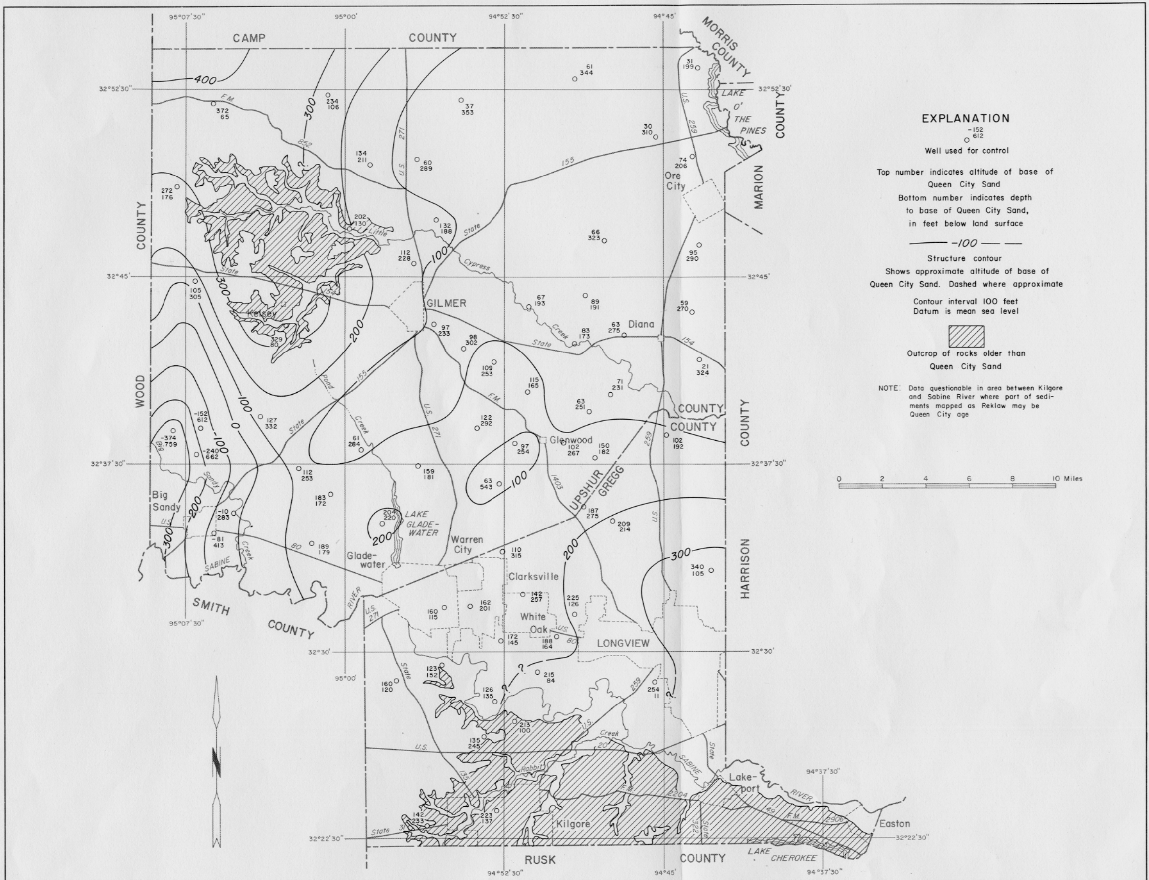
Figure 5 Approximate Altitude of and Depth to the Base of the Queen City Sand
