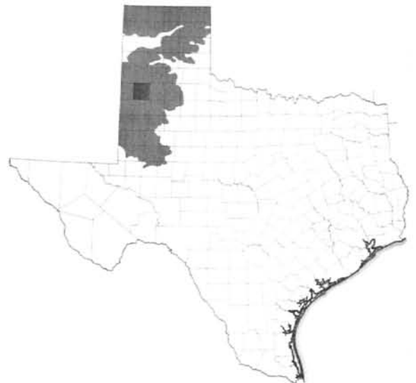
Location of Lamb County, and Extent of the Ogallala Aquifer in Texas
