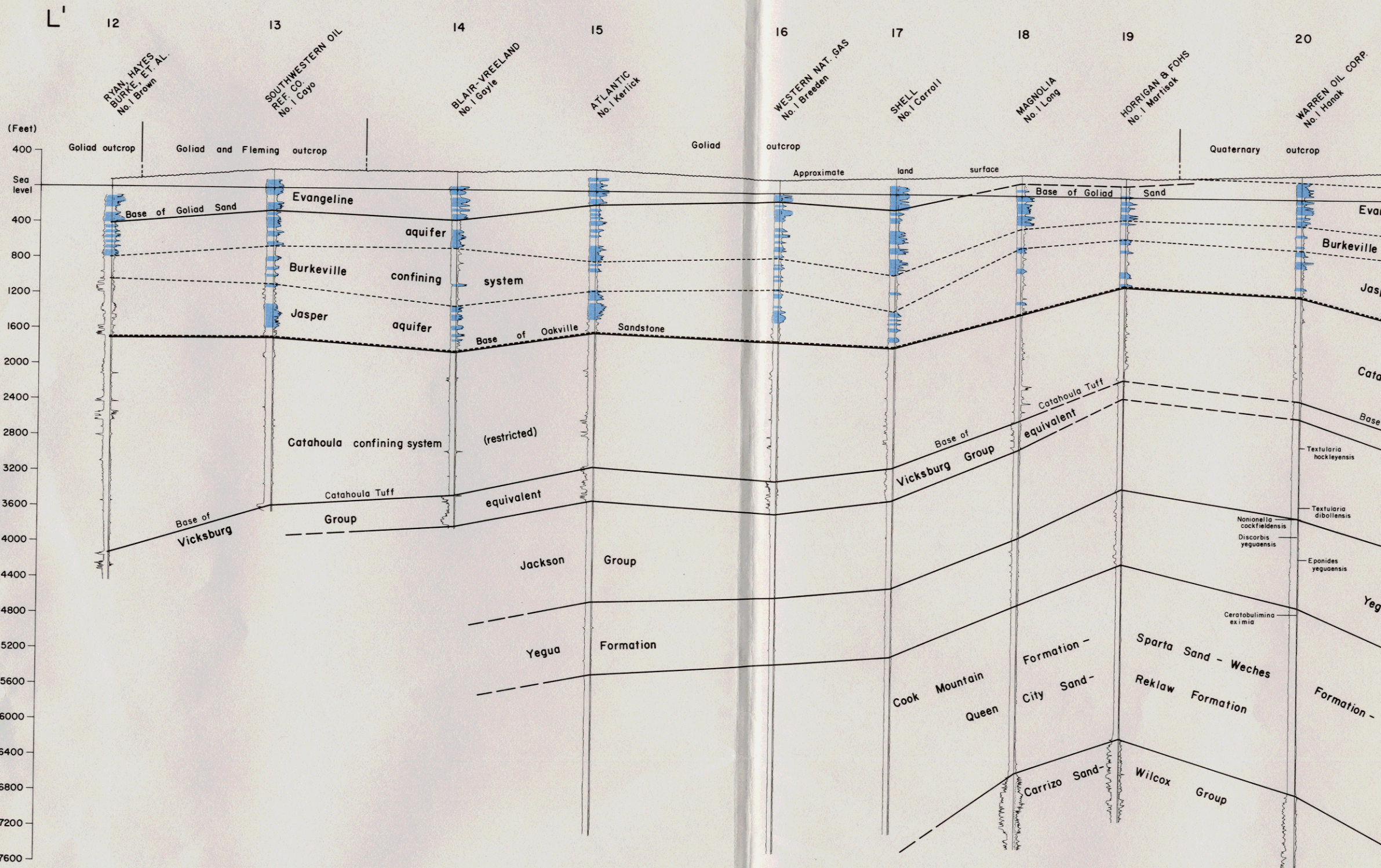
Figure 14 Stratigraphic and Hydrogeologic Section L'-L''
