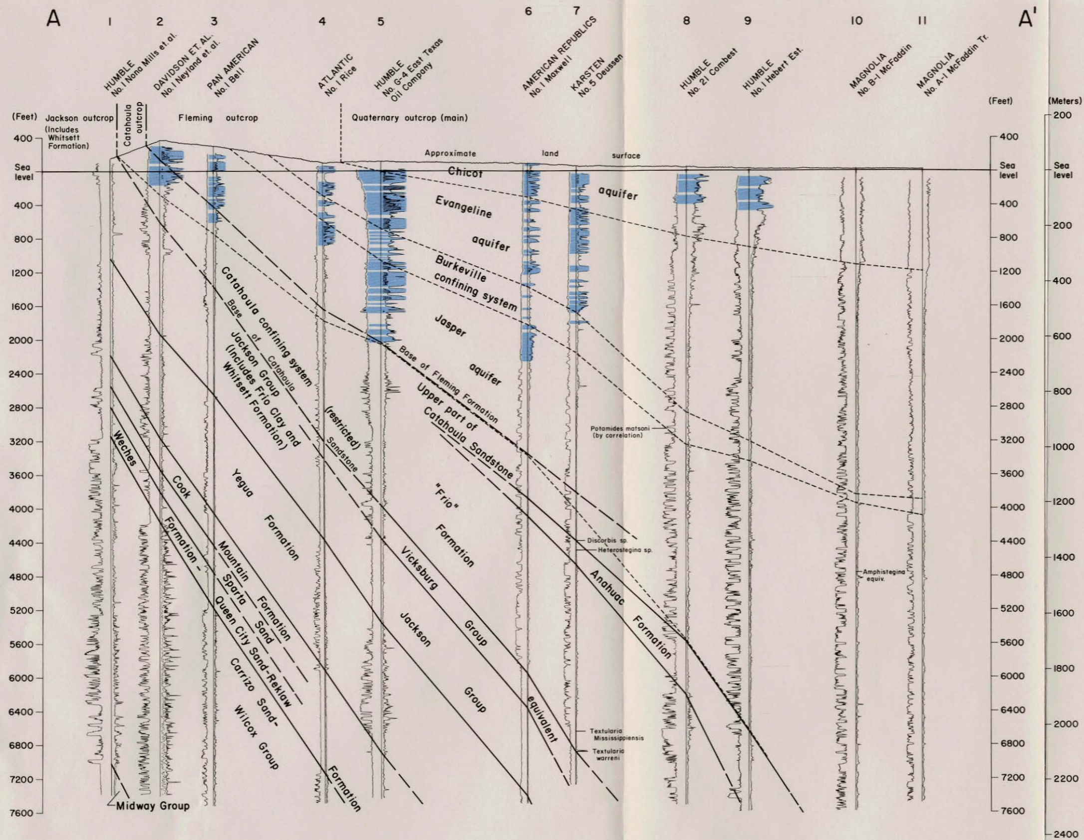
Figure 2 Stratigraphic and Hydrogeologic Section A-A'
