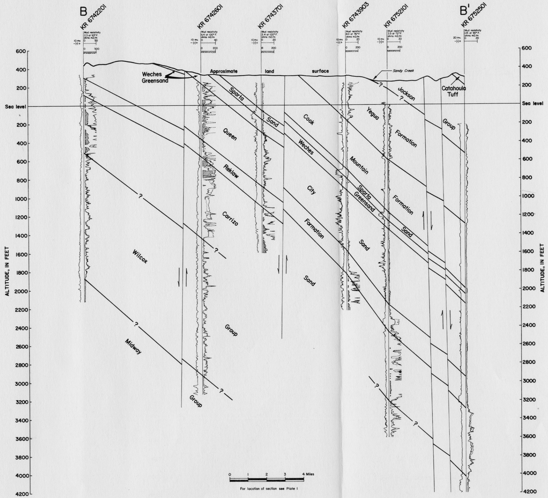
Plate 3 Geologic Section B-B'
