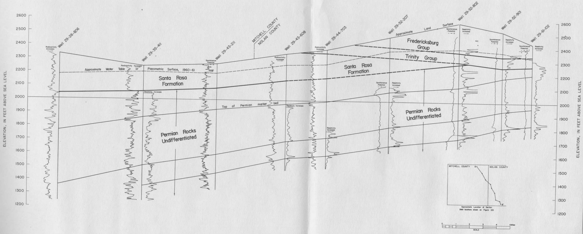
Figure 10 Geologic Section B-B'
