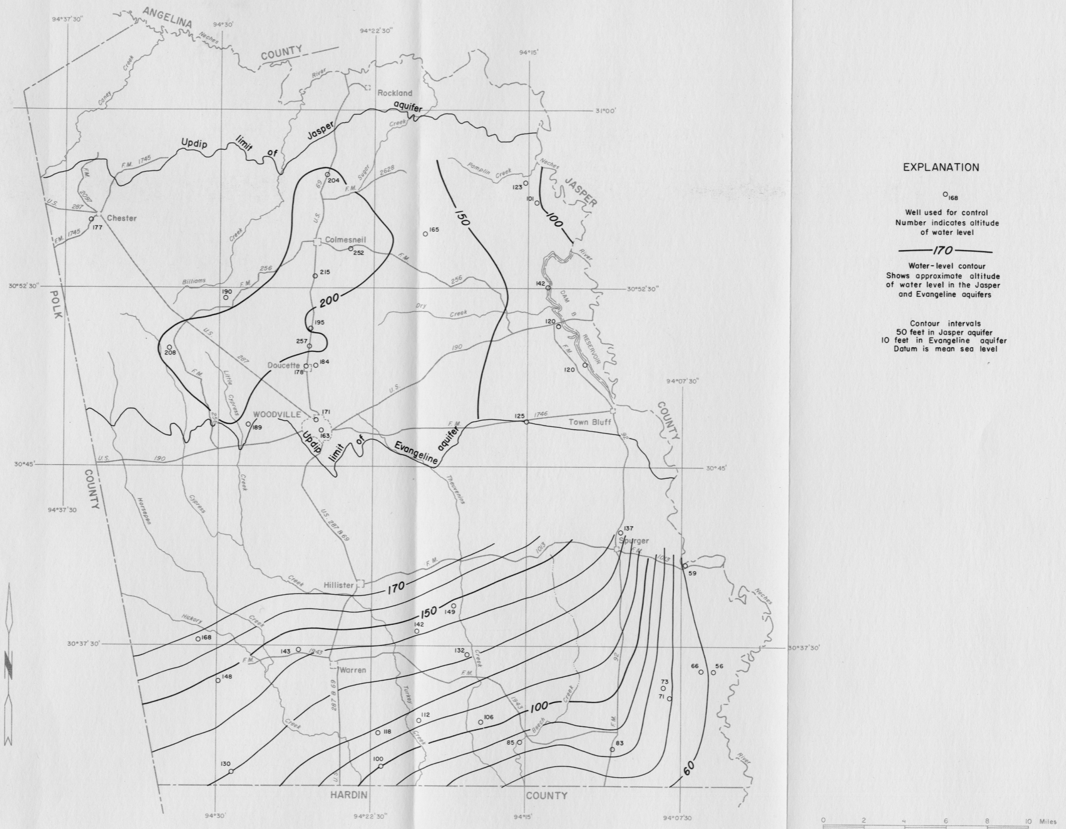
Figure 8 Altitude of Water Levels in Wells Tapping the Jasper and Evangeline Aquifers, 1965
