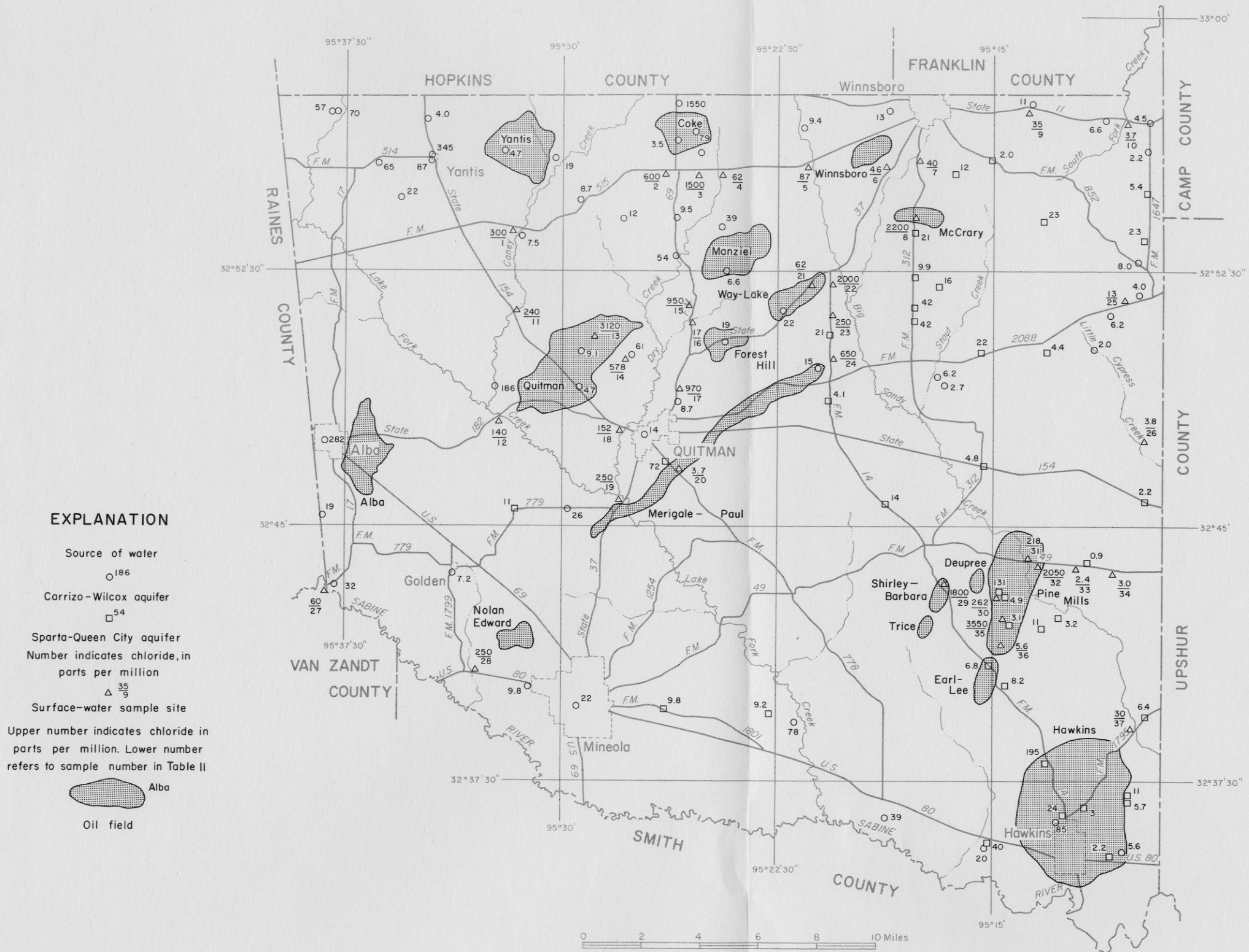
Figure 15 Chloride Content of Water from Selected Wells and Streams and Locations of Oil Fields
