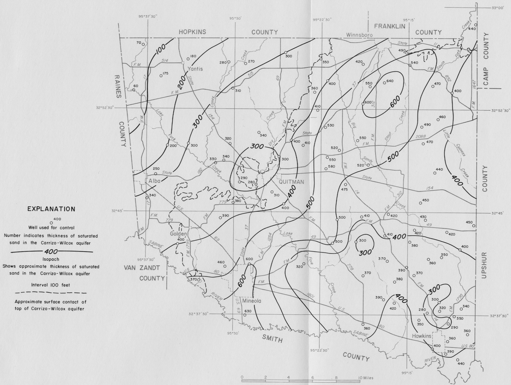
Figure 16 Approximate Thickness of Sand Containing Fresh Water in the Carrizo-Wilcox Aquifer
