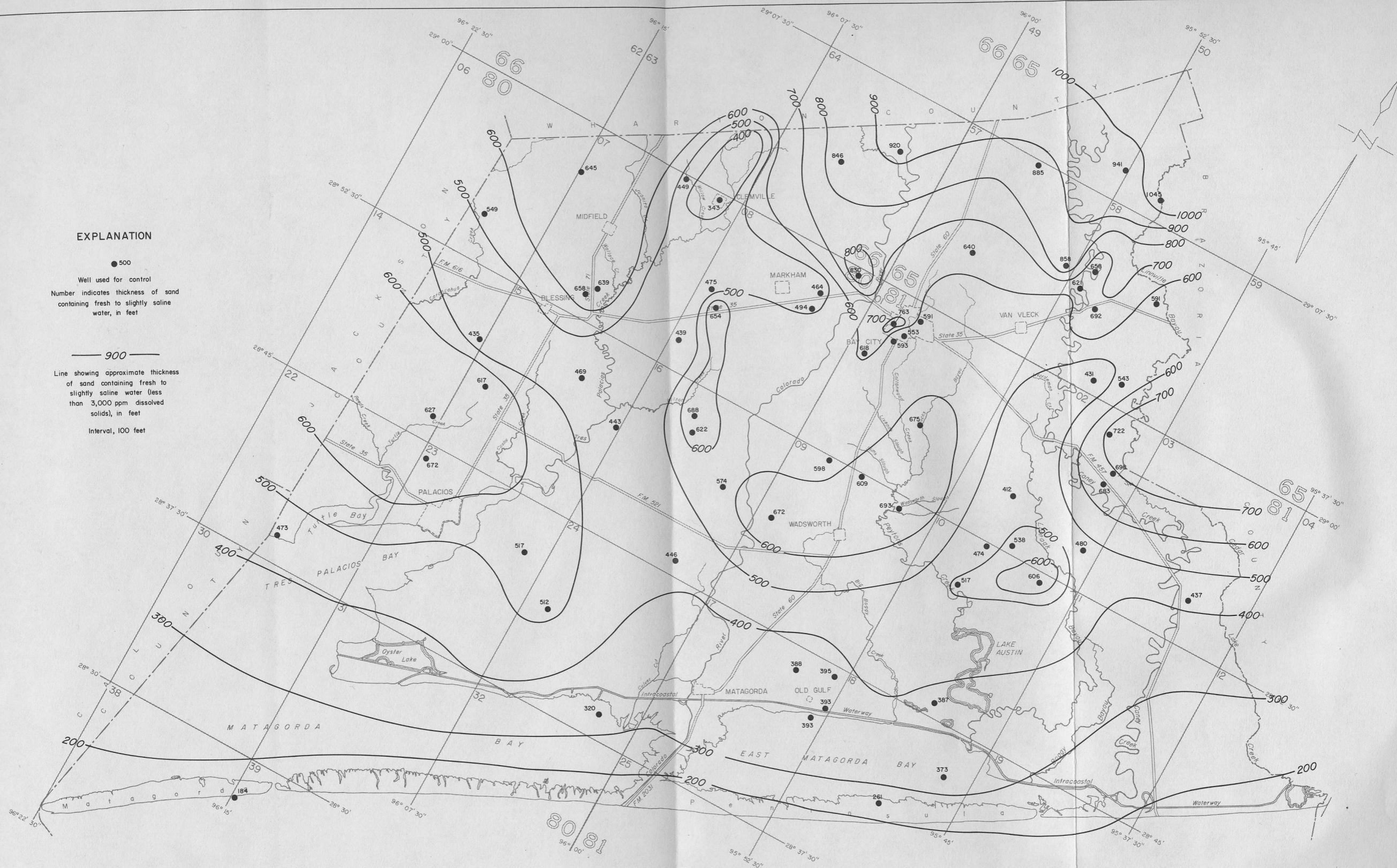
Figure 29 Approximate Thickness of Sand Containing Fresh to Slightly Saline Water (Less than 3,000 ppm Dissolved Solids)
